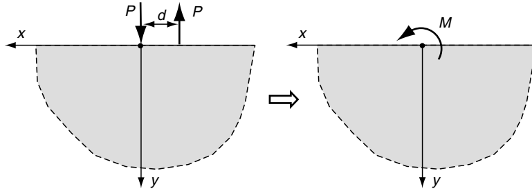
FIGURE 8-23 Half space with concentrated surface moment loading.
