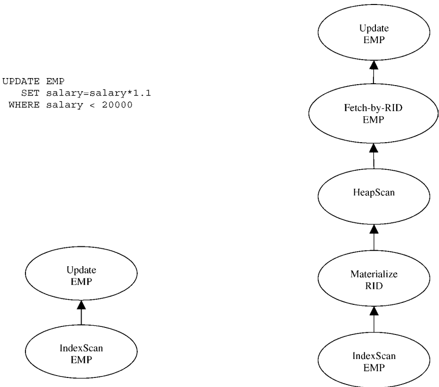
Fig. 4.3 Two query plans for updating a table via an IndexScan. The plan on the left is susceptible to the Halloween problem. The plan on the right is safe, since it identifies all tuples to be updated before actually performing any updates.
