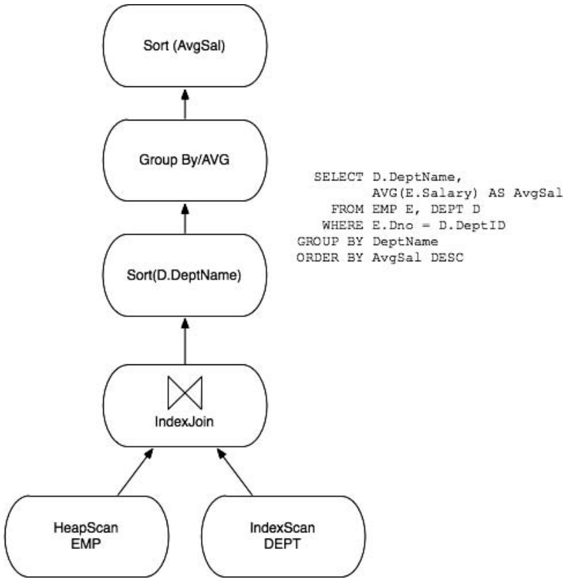
Fig. 4.1 A Query plan. Only the main physical operators are shown.
