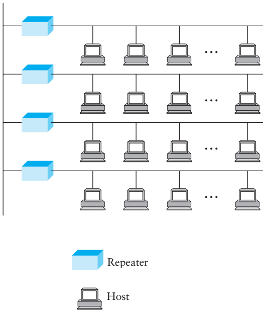
Figure 2.25 Ethernet repeater.
