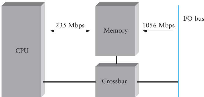
Figure 2.45 Memory bandwidth on a modern PC-class machine.
