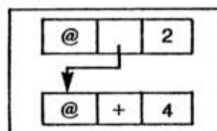
Figure 10.5 The concrete tree of (+ 4 2) (unboxed representations)
